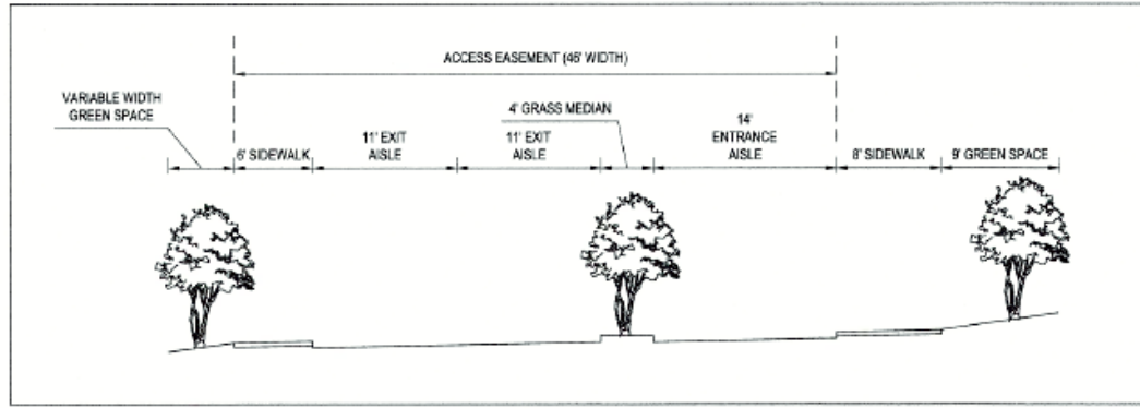
ACCESS EASEMENT 'A' SECTION
