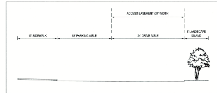
ACCESS EASEMENT 'E' SECTION
