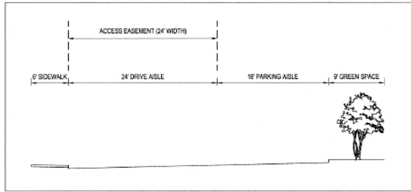
ACCESS EASEMENT 'C' SECTION
