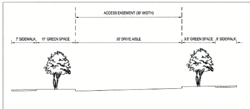
ACCESS EASEMENT 'B' SECTION
