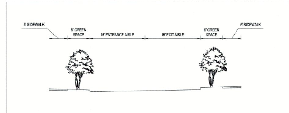
ACCESS EASEMENT 'G' SECTION
