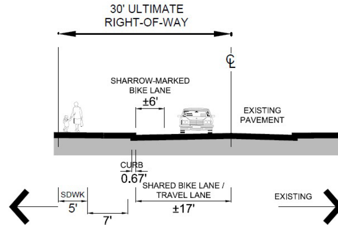
URBAN PRMIARY RESIDENTIAL ROAD STD -100.06 MANNING ROAD - HALF SECTION
