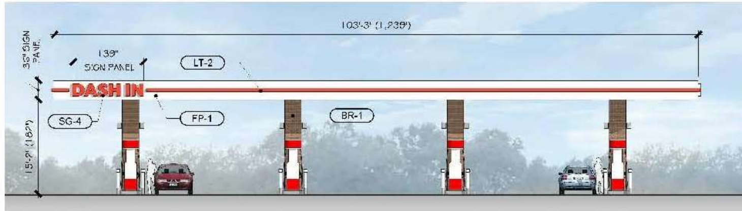
Front (East) Elevation
