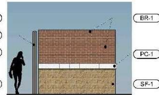
Side Elevation (NTS)
