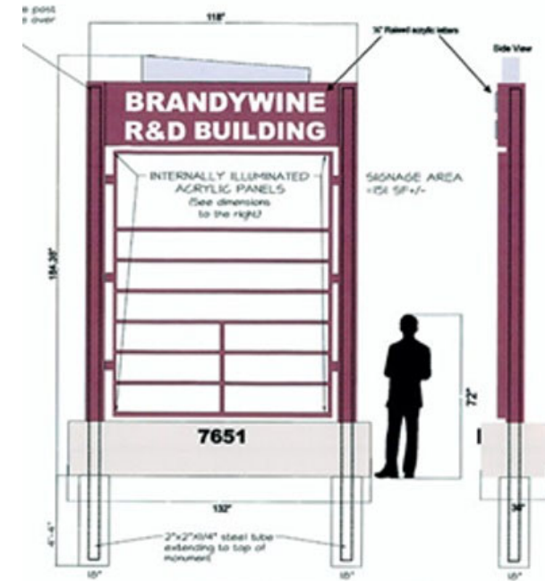
2 FREE STANDING SIGN ELEVATION NO SCALE
