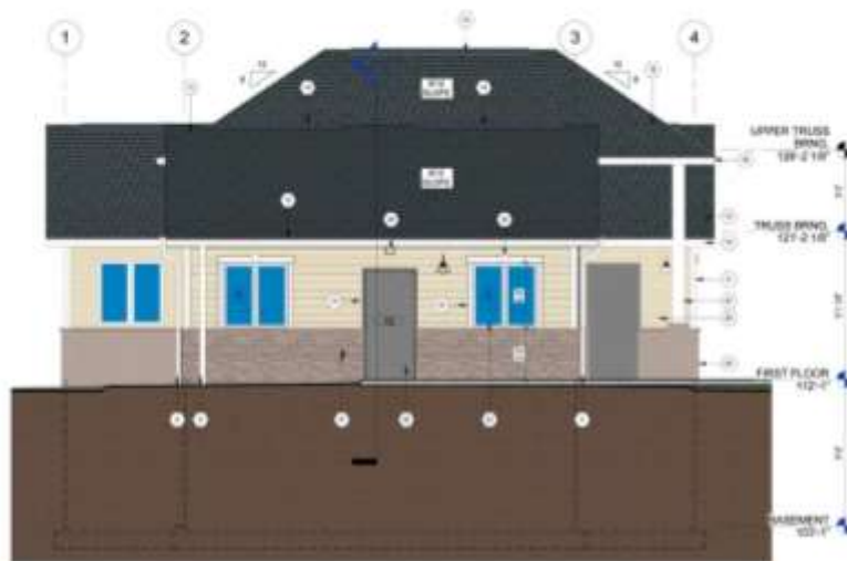
1 EXTERIOR ELEVATION - NORTH (FRONT)
