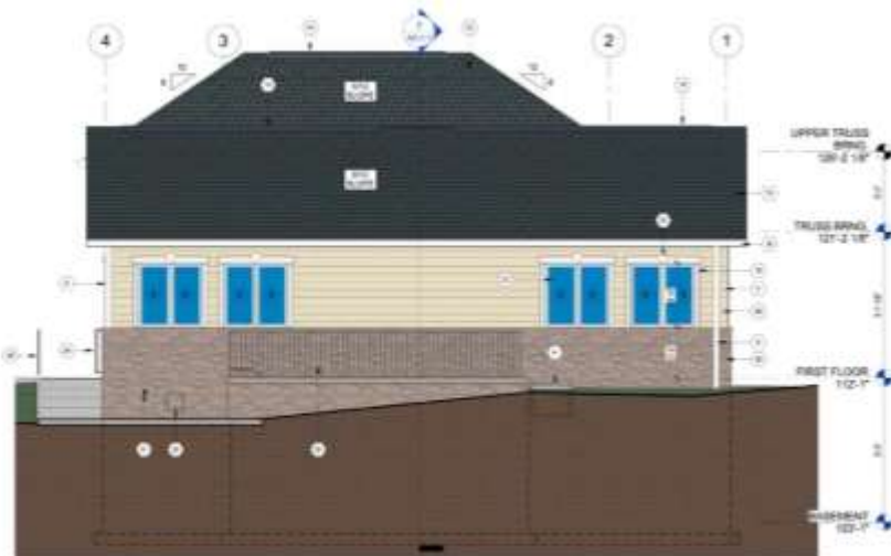
EXTERIOR ELEVATION - WEST
