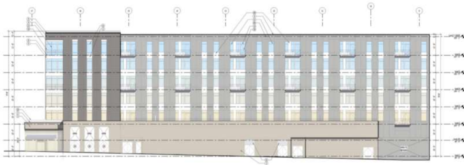
BUILDING 1 ELEVATION - NORTH - NEW ALLEY
