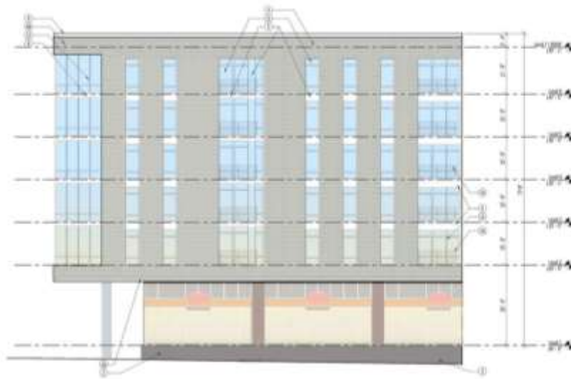
BUILDING 2 ELEVATION - WEST - GUILFORD DR.
