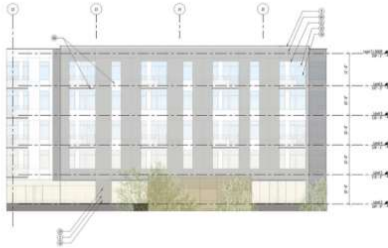
BUILDING 2 ELEVATION - COURTYARD SOUTH DRP 17-003
