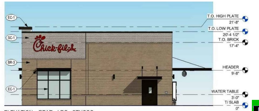
ELEVATION - REAR - LRG - STUCCO 1/8" = 1'-0"
