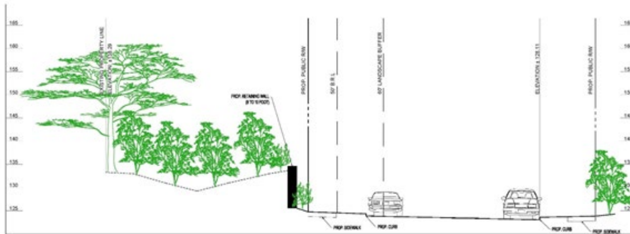
PROFILE B-B'
