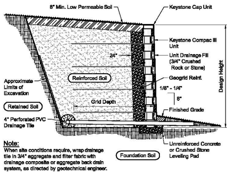
4 TYPICAL REINFORCED WALL SECTION
