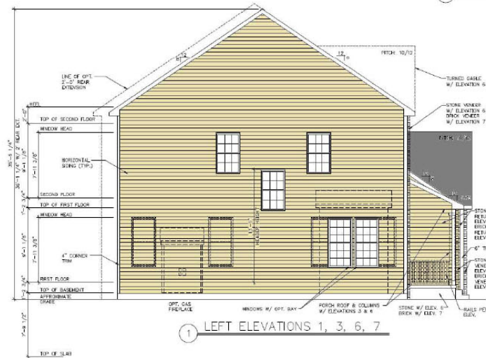
1 REAR ELEVATION
