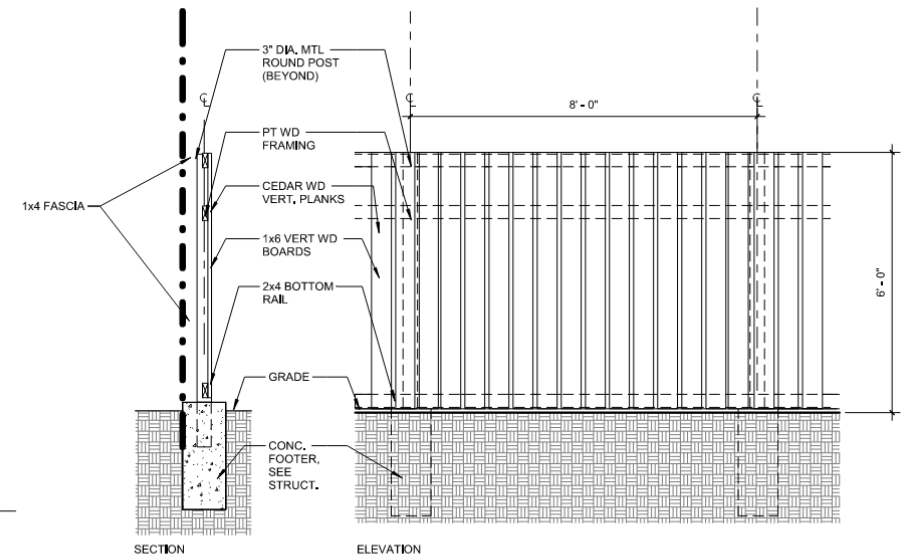
2 W1 - FENCE DETAIL 1/2" = 1'-0"
