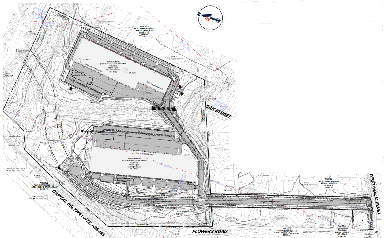
Figure 1: Site Plan
