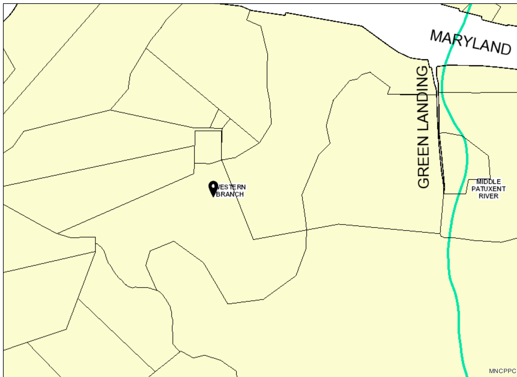
Figure 6 - Watershed Map
